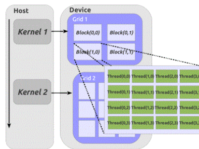
Fig.4 Decomposition of blocks of grid data, where each block contains a number of elements executed in parallel. The term defines the Host CPU and Device term corresponds to the GPU. The size used for the definition of the grid is two-dimensional block-level and threads.
