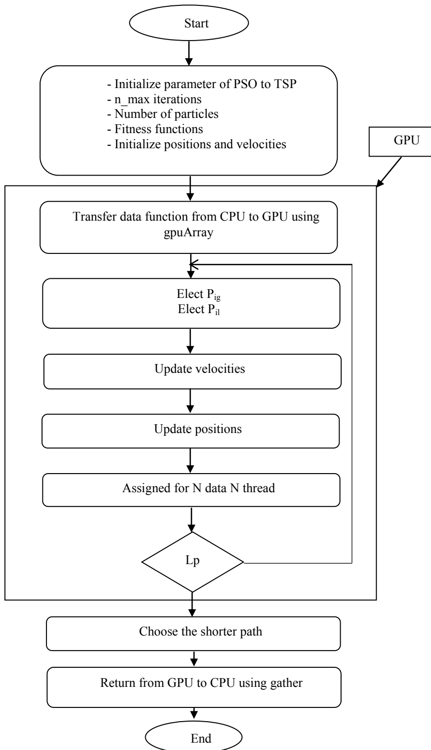
Fig.5. The process of GPU-PSO-A-TSP
