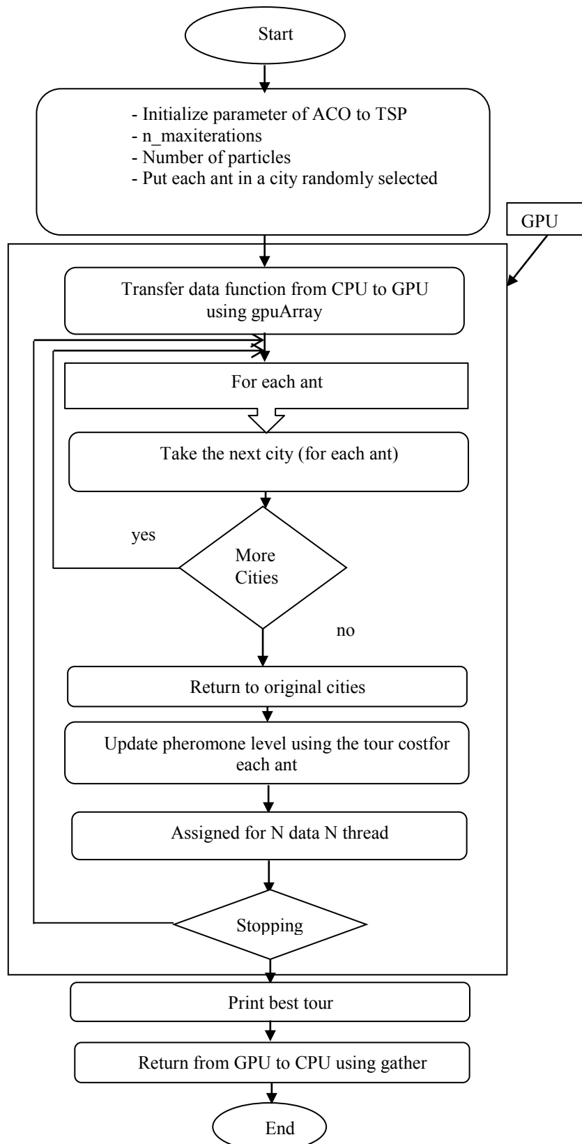
Fig.6. The process of GPU-ACO-A-TSP
